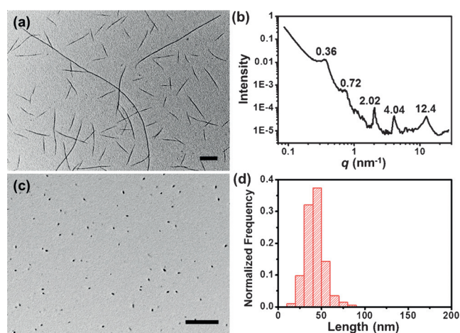
Figure 1. a) TEM images of the cylindrical micelles formed by dispersing P2VP 68 - b -PFMA 41 into i -PrOH (0.5 mg mL -1 ) at 80 °C for 1 h and cooling to 23 °C; b) spliced small, medium, and wide X-ray scattering spectra of dried cylindrical micelle sample shown in (a); c) the seeds obtained by ultrasonication of the cylindrical micelle solution in i -PrOH at 0 °C for 4 h; d) contour length distribution of the seeds in (c), L_n = 42 nm, L_w = 45 nm, L_w/L_n = 1.07 . Scale bars are 500 nm.
